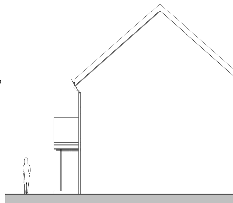
West Elevation
